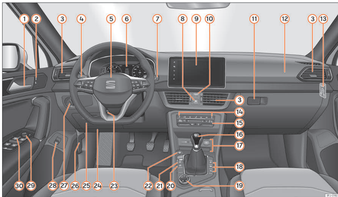
Fig. 53 Cockpit
