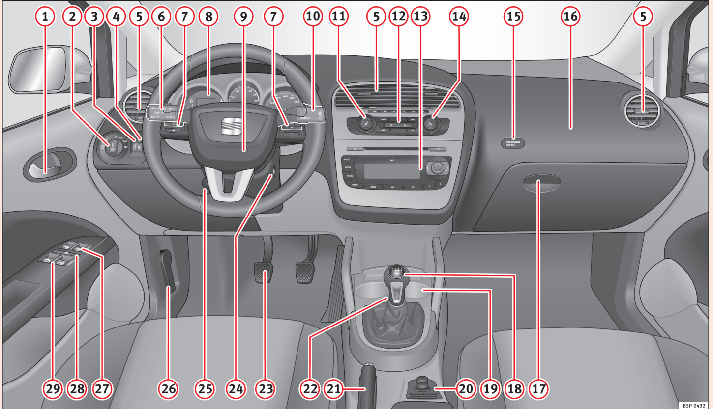
Fig. 32 Instrumentpanel
